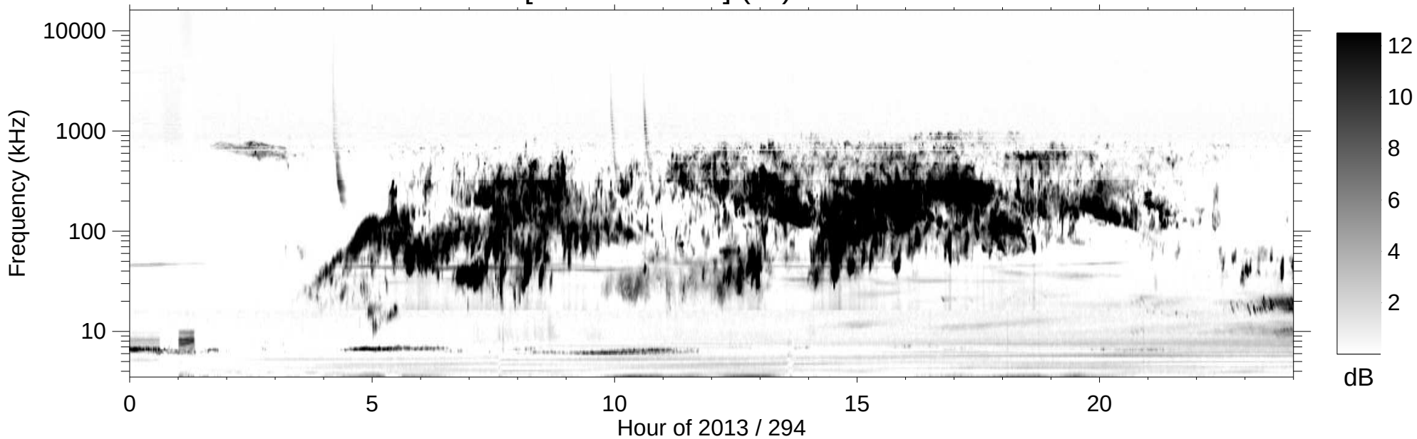
RPWS [ABCH1H2/Ex] (-B) 2013/10/21
