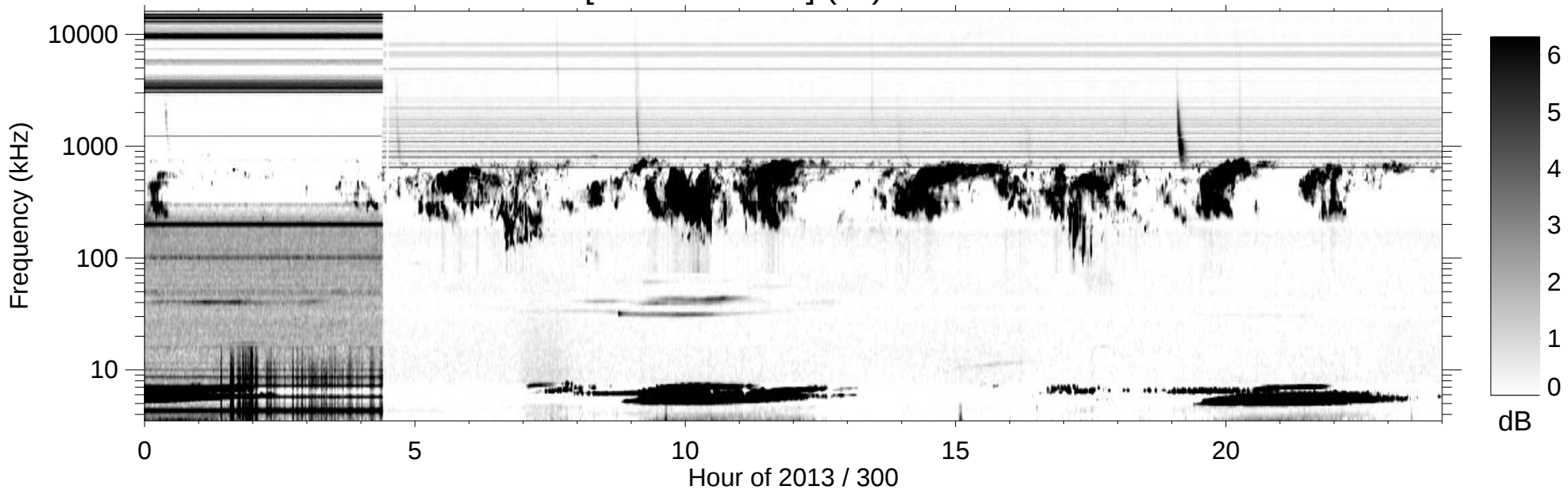
RPWS [ABCH1H2/Ex] (-B) 2013/10/27
