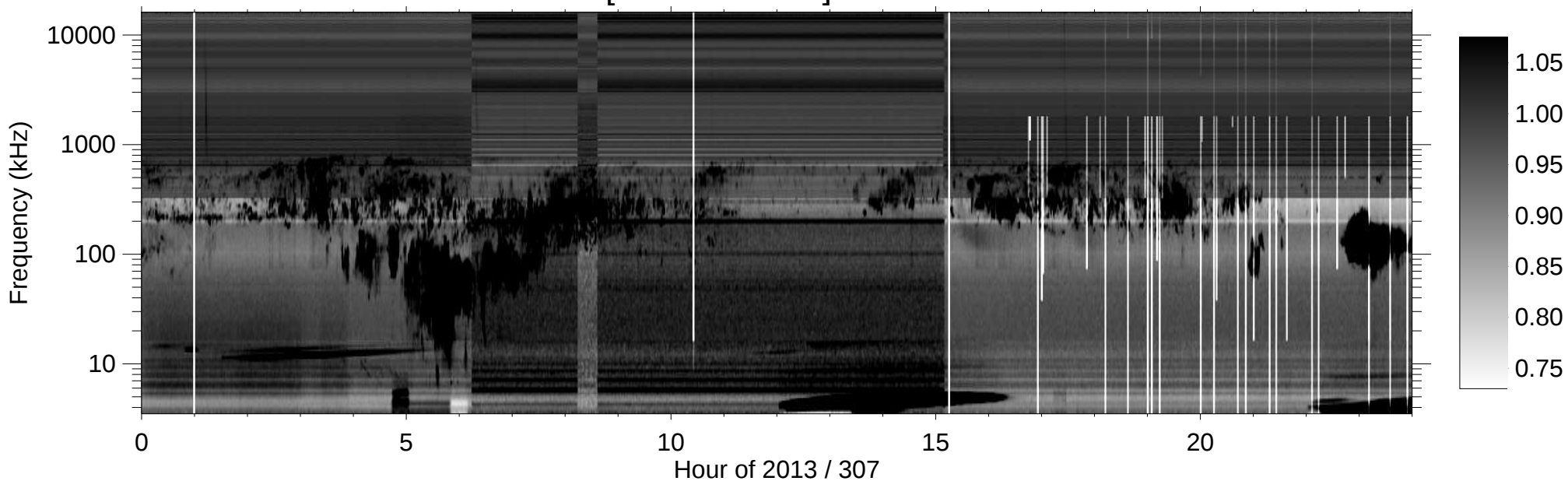
RPWS [ABCH1H2/Ex] (-B) 2013/11/03
