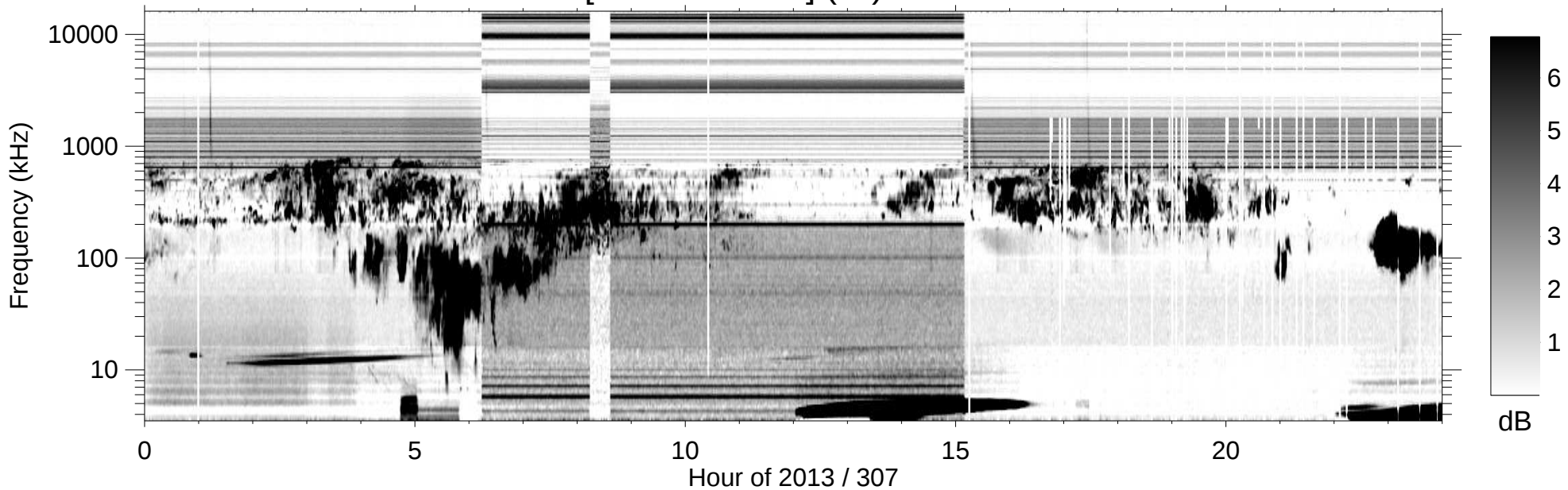
RPWS [ABCH1H2/Ex] (-B) 2013/11/03
