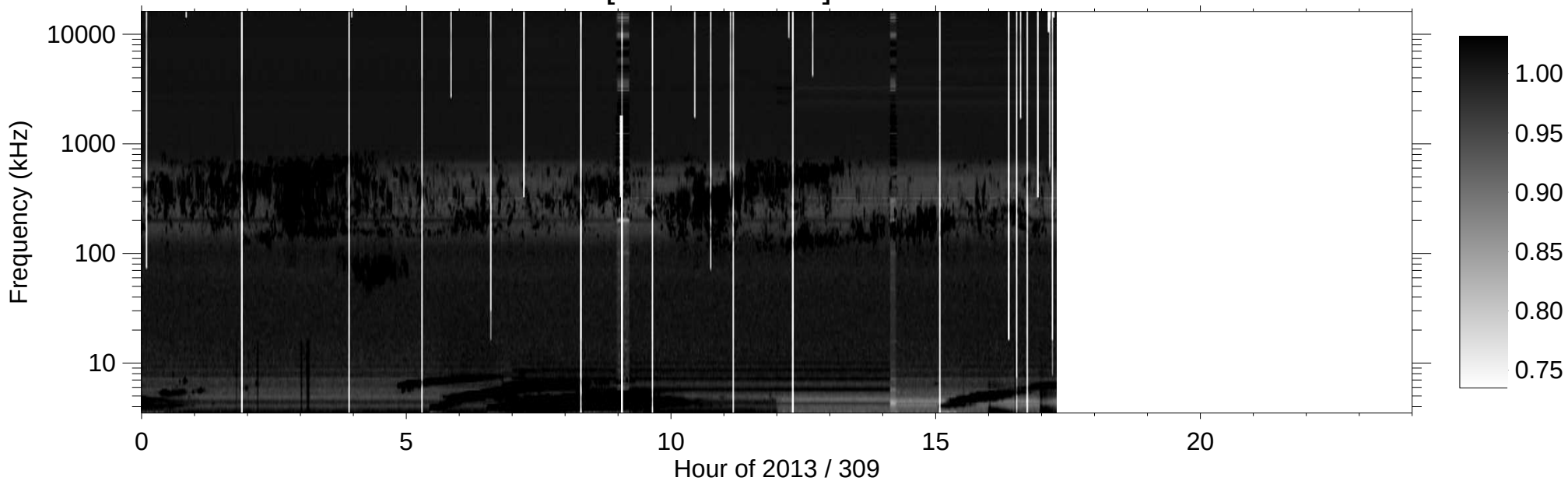
RPWS [ABCH1H2/Ex] (-B) 2013/11/05
