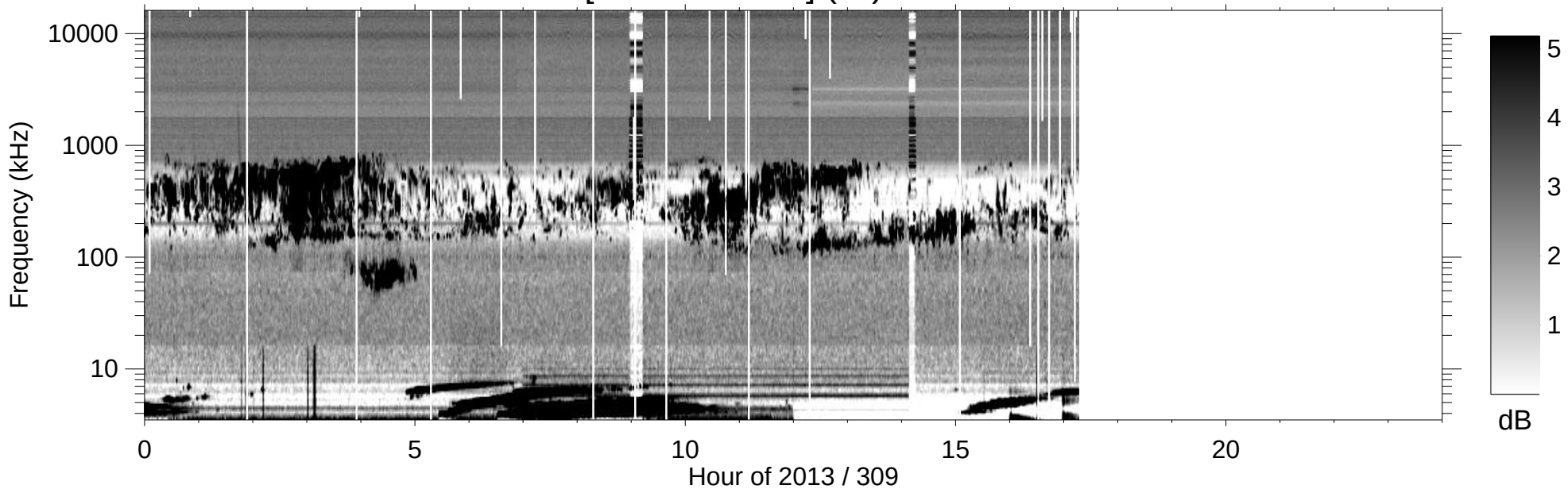
RPWS [ABCH1H2/Ex] (-B) 2013/11/05
