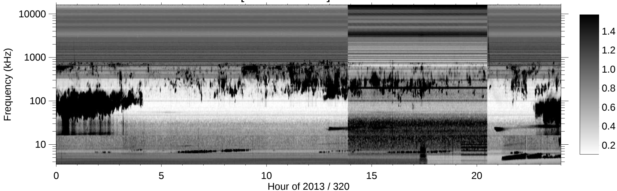
RPWS [ABCH1H2/Ex] (-B) 2013/11/16
