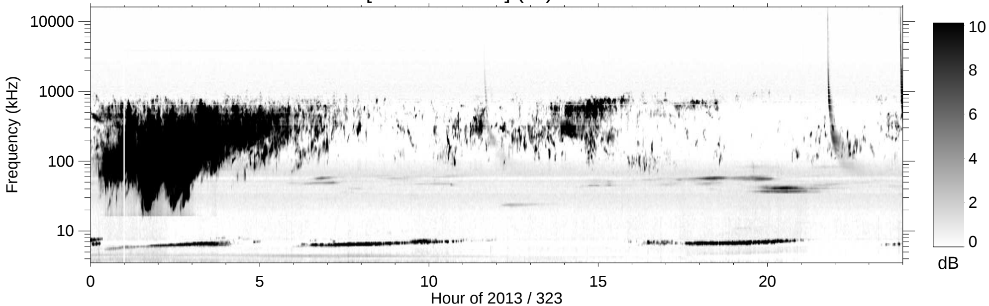
RPWS [ABCH1H2/Ex] (-B) 2013/11/19
