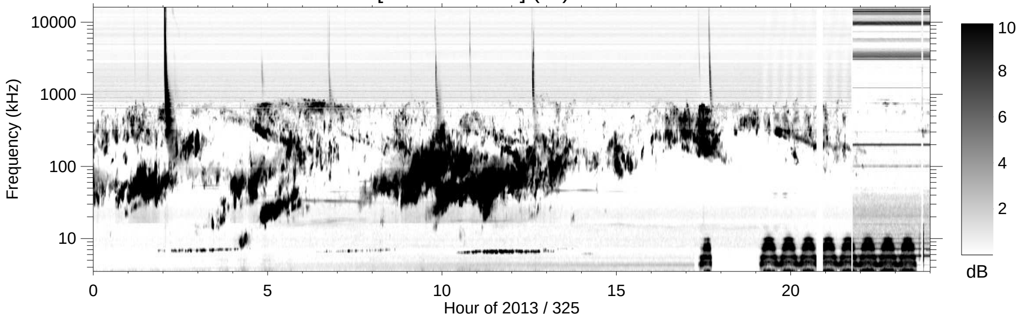
RPWS [ABCH1H2/Ex] (-B) 2013/11/21
