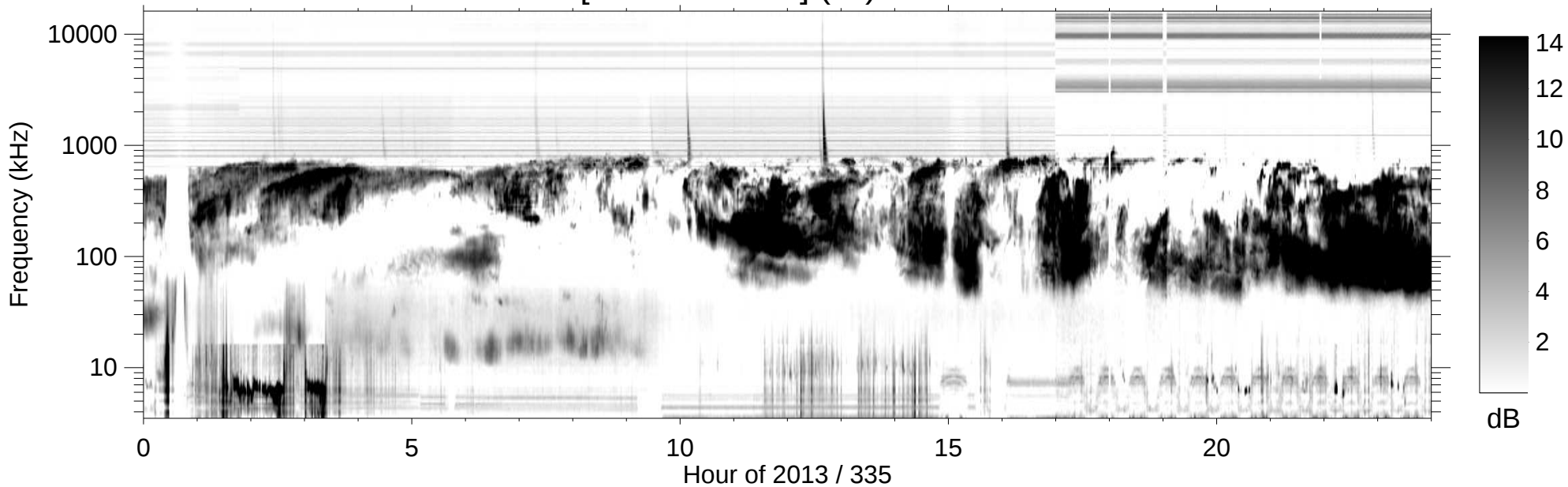
RPWS [ABCH1H2/Ex] (-B) 2013/12/01
