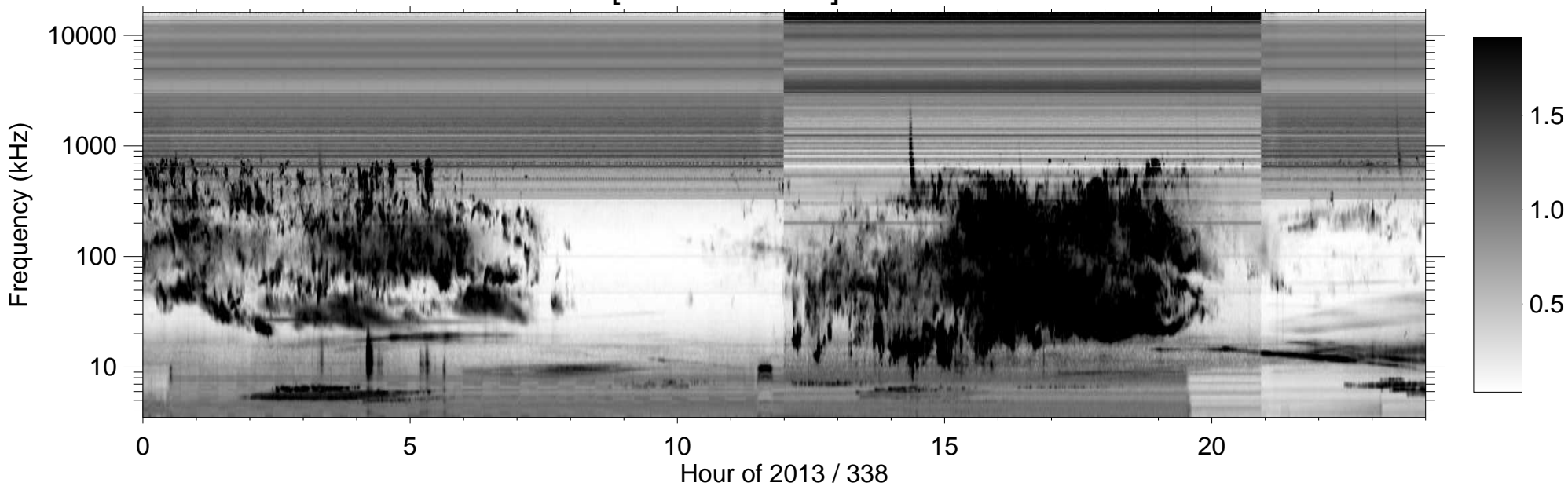
RPWS [ABCH1H2/Ex] (-B) 2013/12/04
