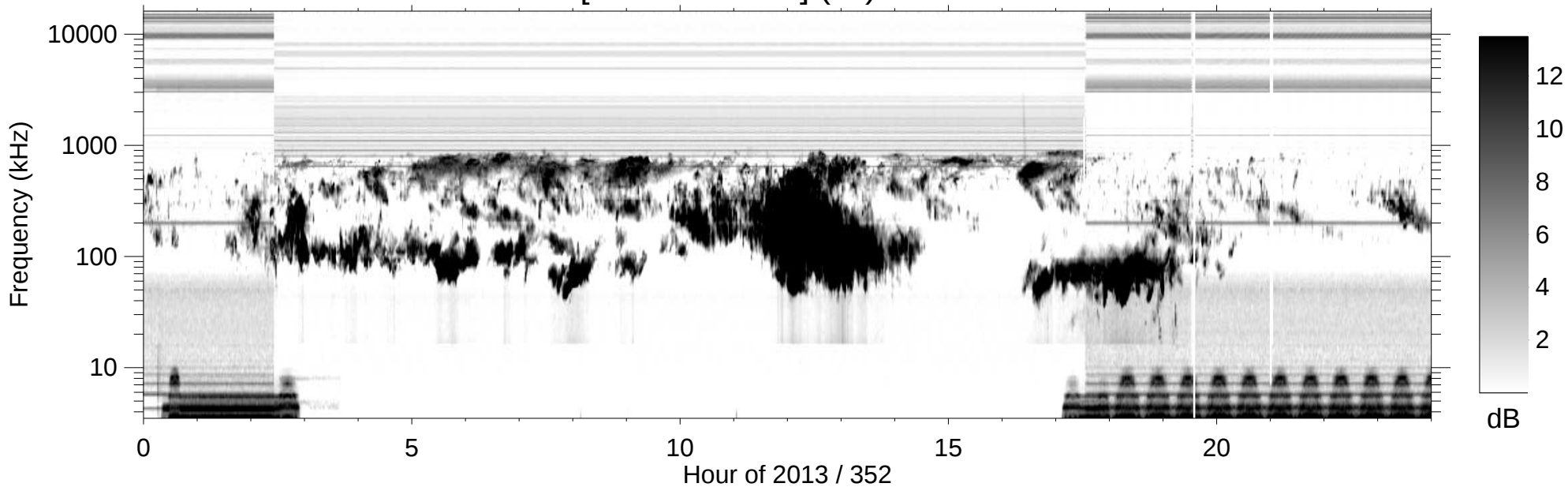
RPWS [ABCH1H2/Ex] (-B) 2013/12/18
