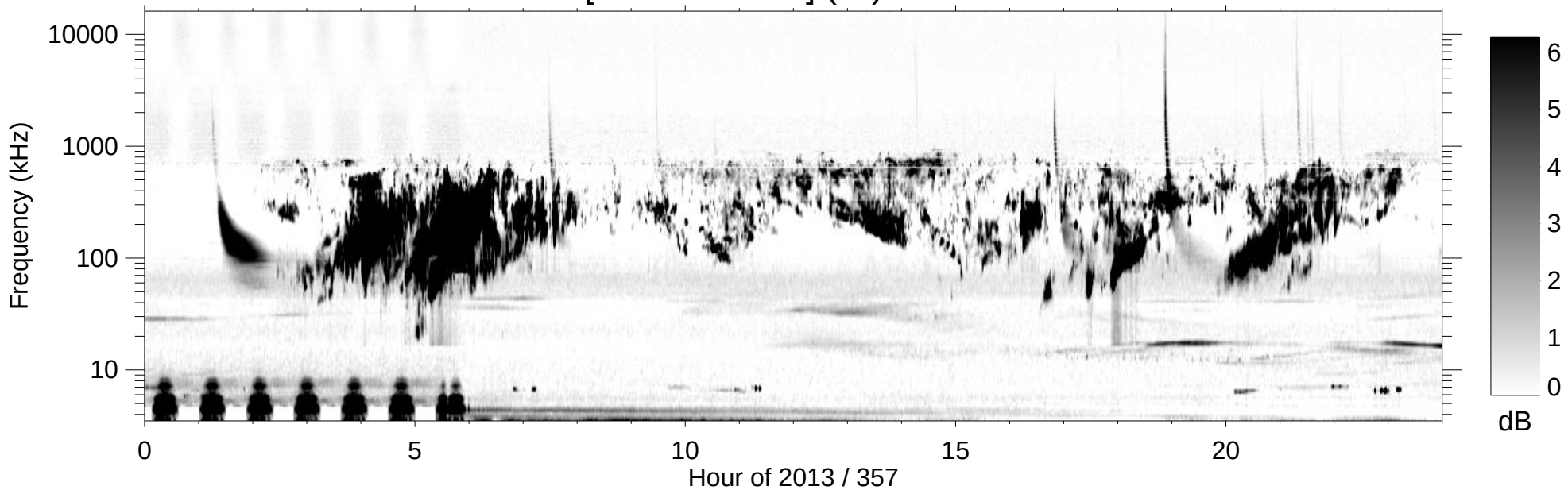
RPWS [ABCH1H2/Ex] (-B) 2013/12/23
