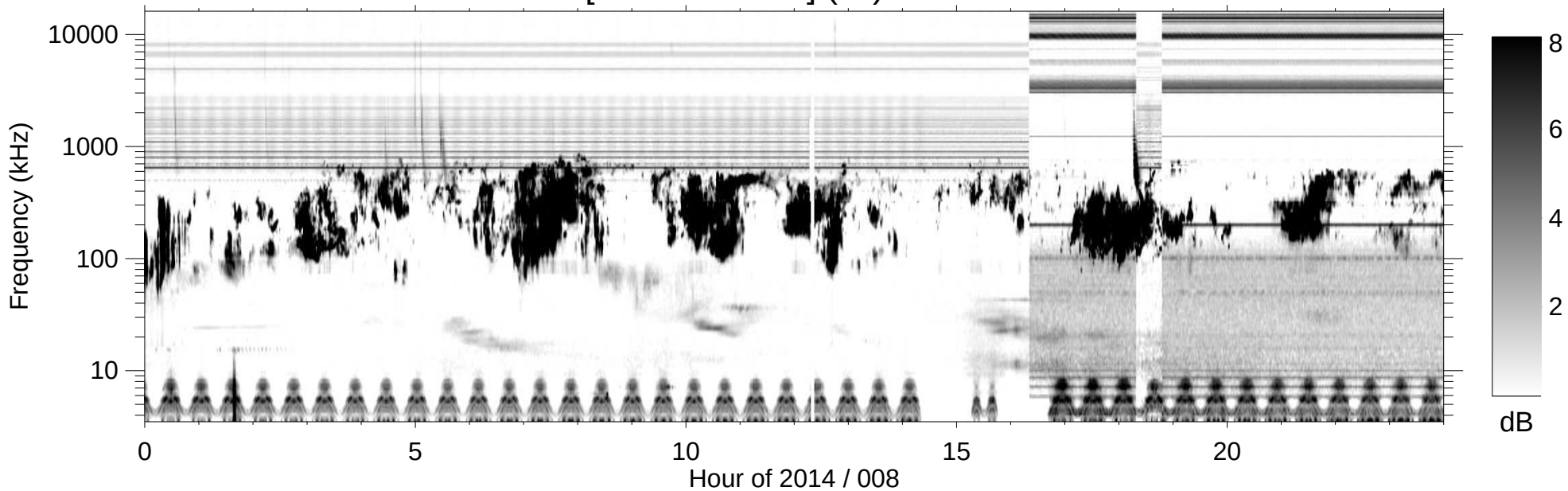
RPWS [ABCH1H2/Ex] (-B) 2014/01/08
