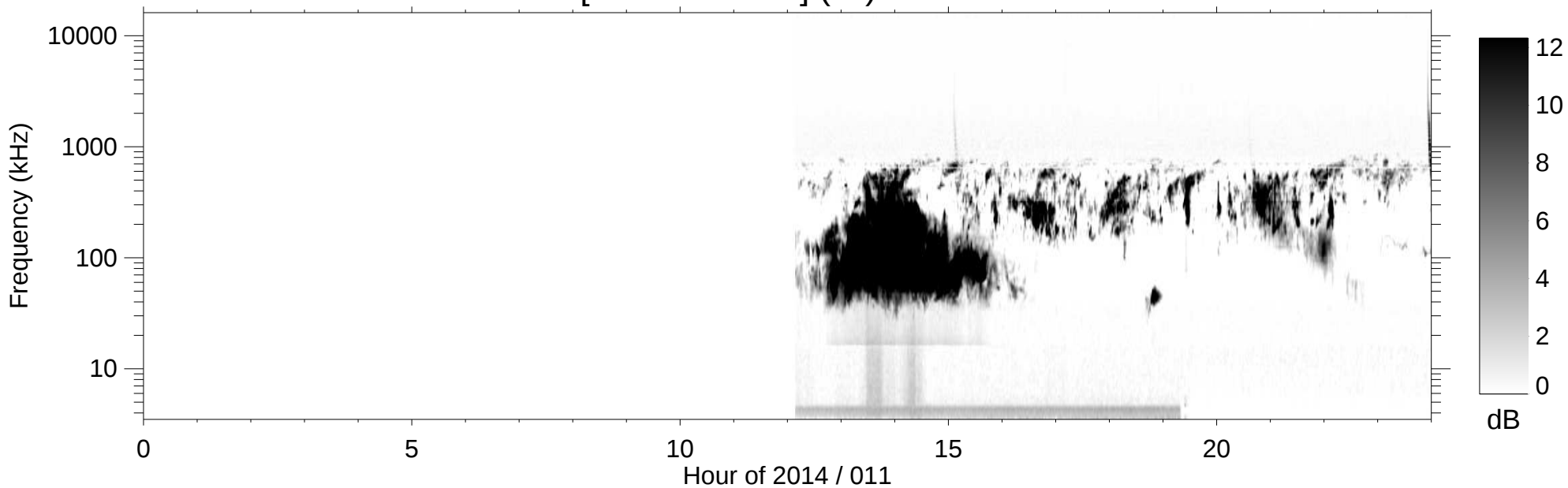
RPWS [ABCH1H2/Ex] (-B) 2014/01/11
