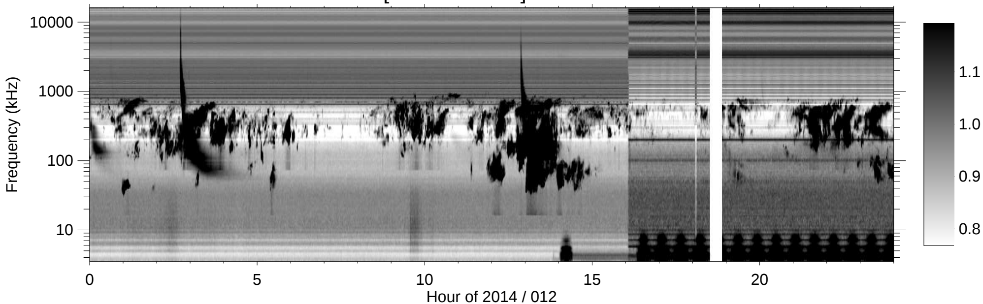
RPWS [ABCH1H2/Ex] (-B) 2014/01/12
