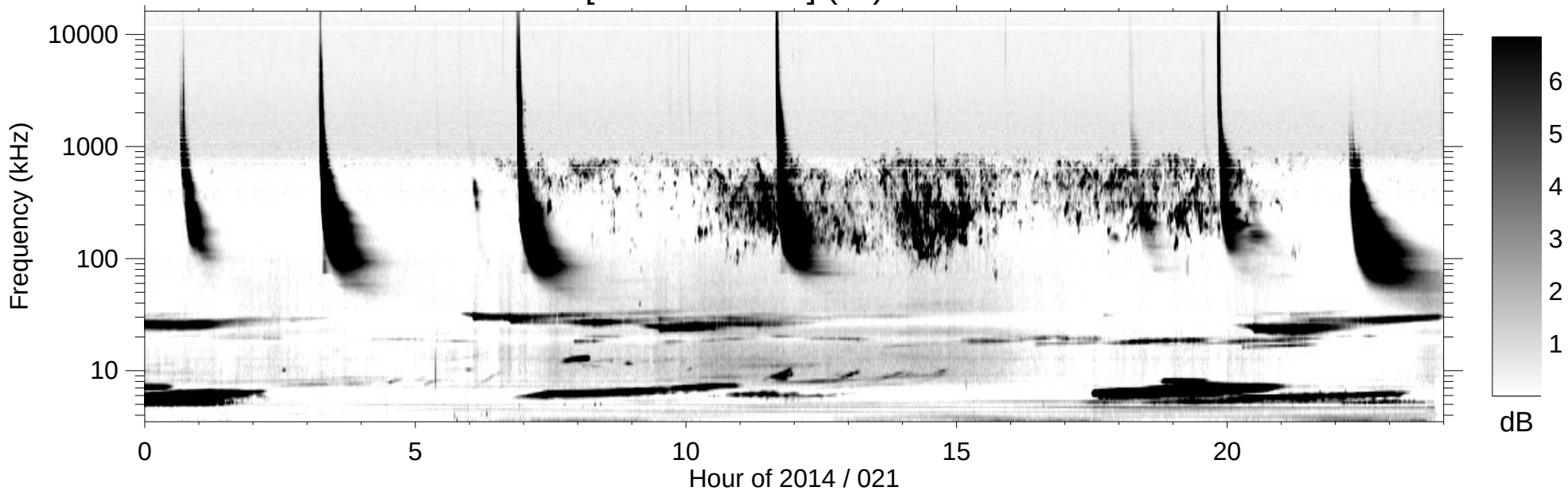
RPWS [ABCH1H2/Ex] (-B) 2014/01/21
