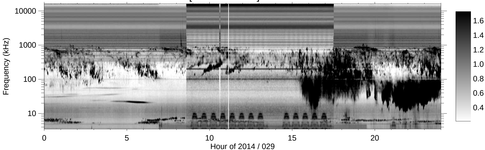
RPWS [ABCH1H2/Ex] (-B) 2014/01/29
