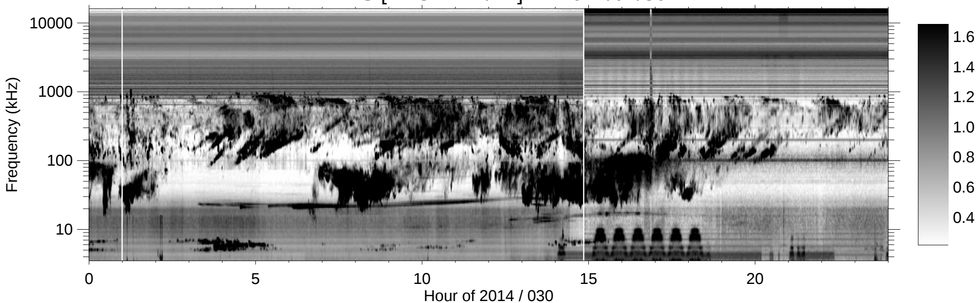
RPWS [ABCH1H2/Ex] (-B) 2014/01/30
