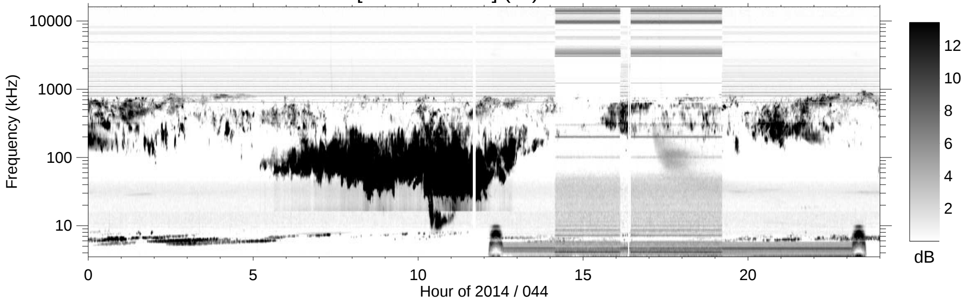
RPWS [ABCH1H2/Ex] (-B) 2014/02/13
