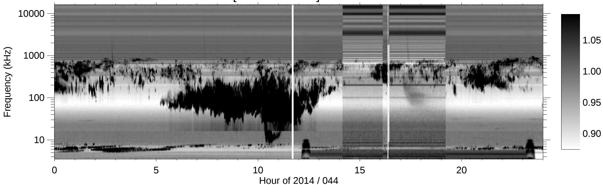
RPWS [ABCH1H2/Ex] (-B) 2014/02/13
