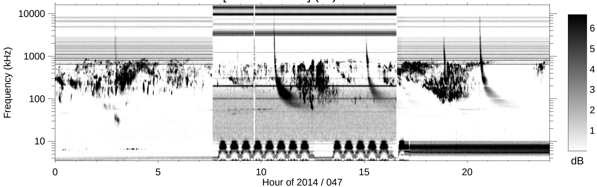
RPWS [ABCH1H2/Ex] (-B) 2014/02/16
