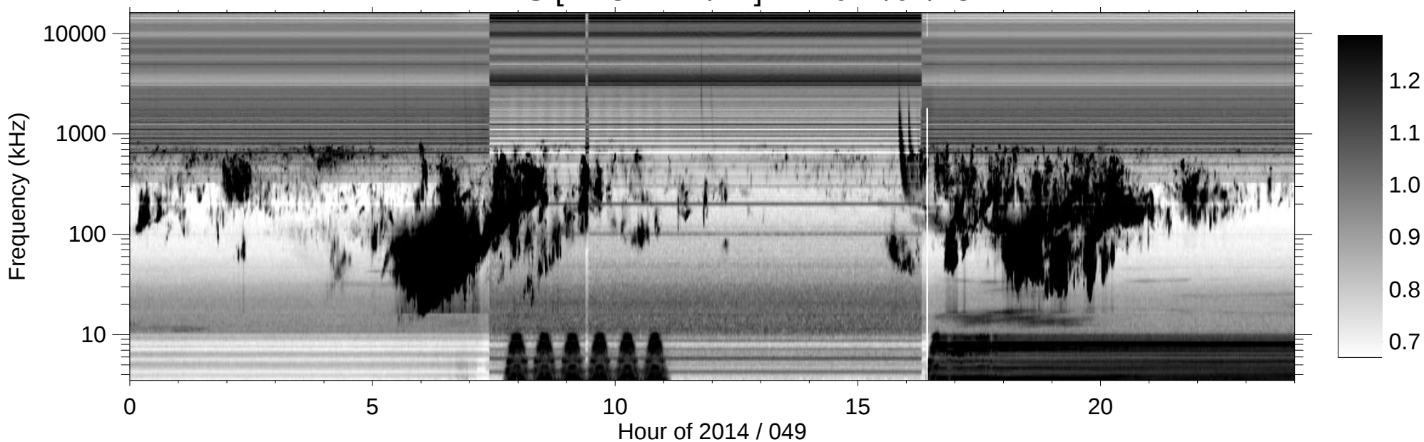
RPWS [ABCH1H2/Ex] (-B) 2014/02/18
