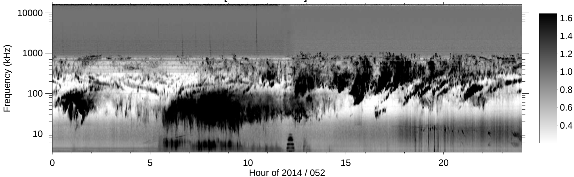
RPWS [ABCH1H2/Ex] (-B) 2014/02/21
