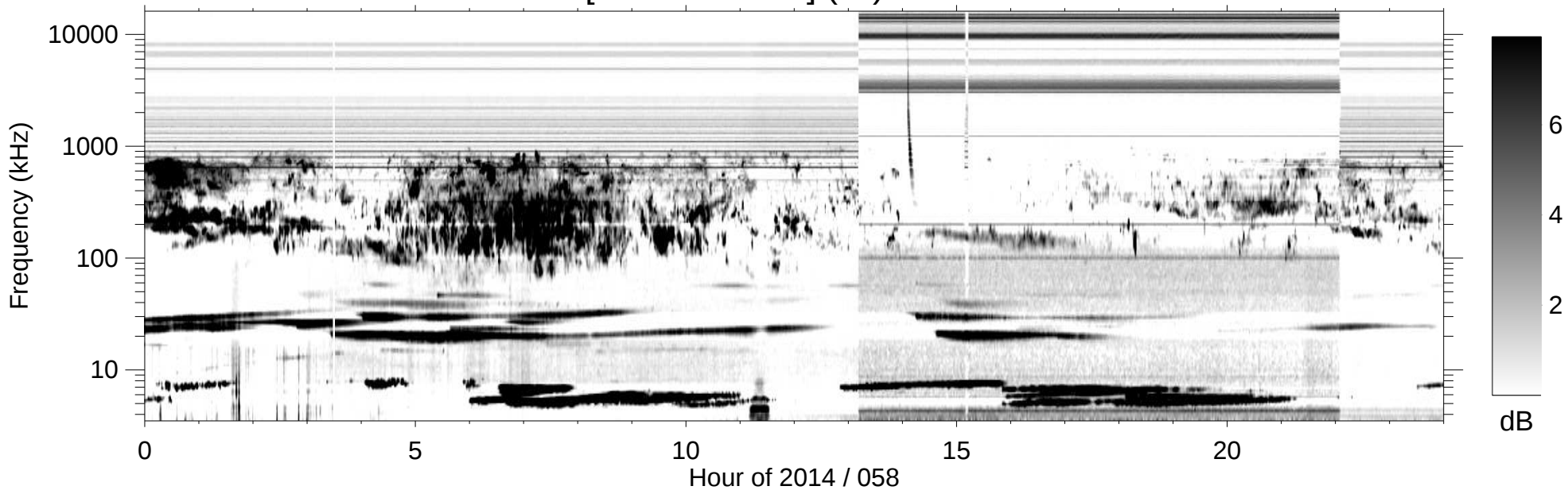
RPWS [ABCH1H2/Ex] (-B) 2014/02/27
