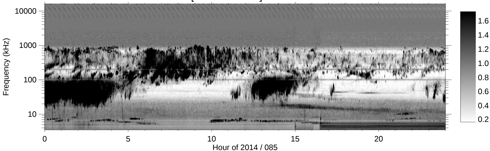
RPWS [ABCH1H2/Ex] (-B) 2014/03/26
