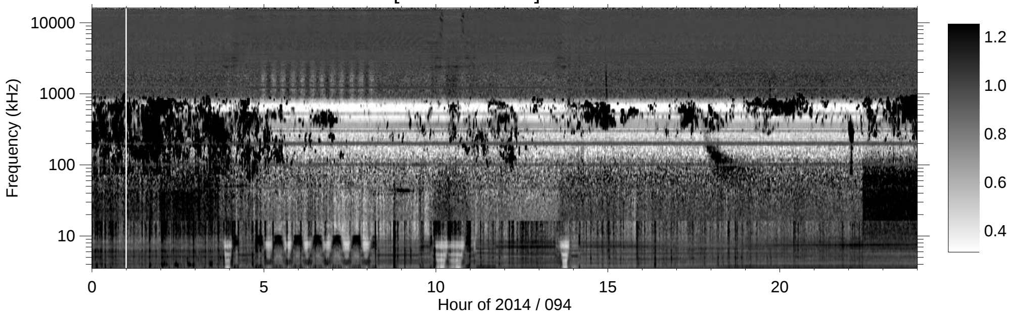
RPWS [ABCH1H2/Ex] (-B) 2014/04/04
