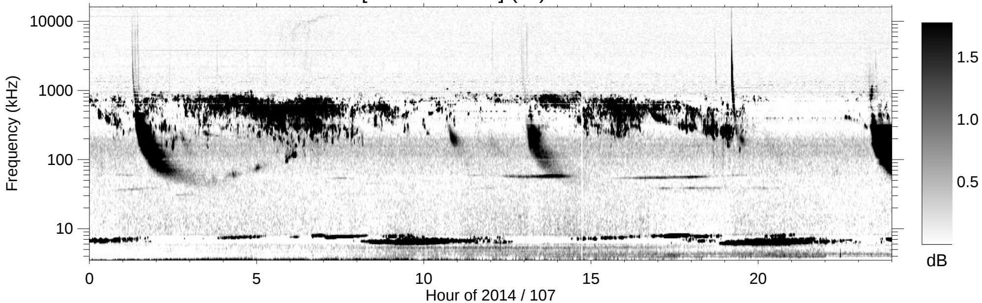
RPWS [ABCH1H2/Ex] (-B) 2014/04/17
