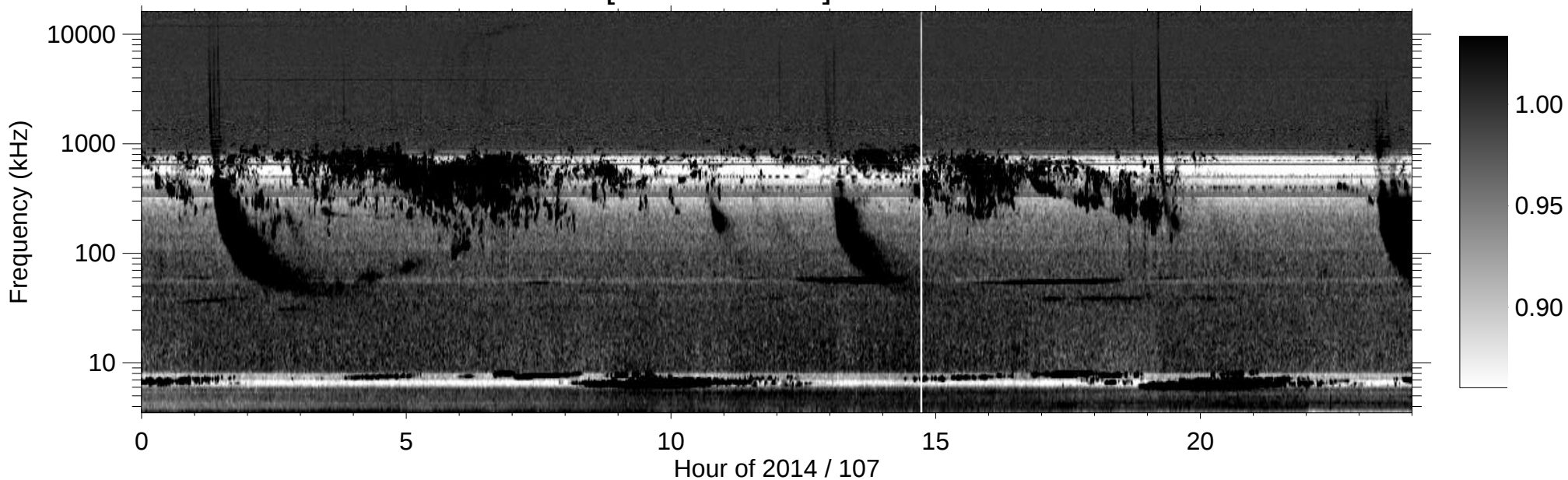
RPWS [ABCH1H2/Ex] (-B) 2014/04/17
