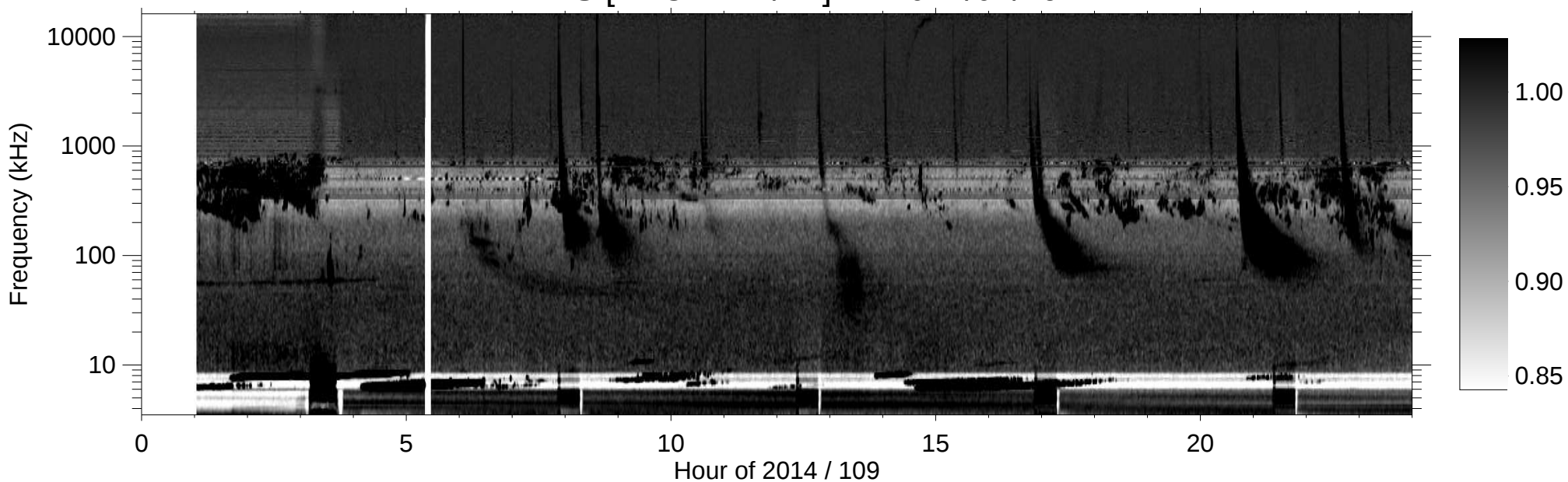
RPWS [ABCH1H2/Ex] (-B) 2014/04/19
