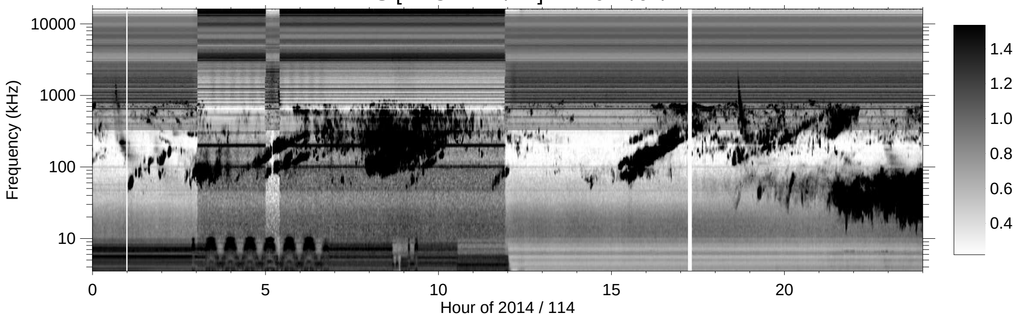
RPWS [ABCH1H2/Ex] (-B) 2014/04/24
