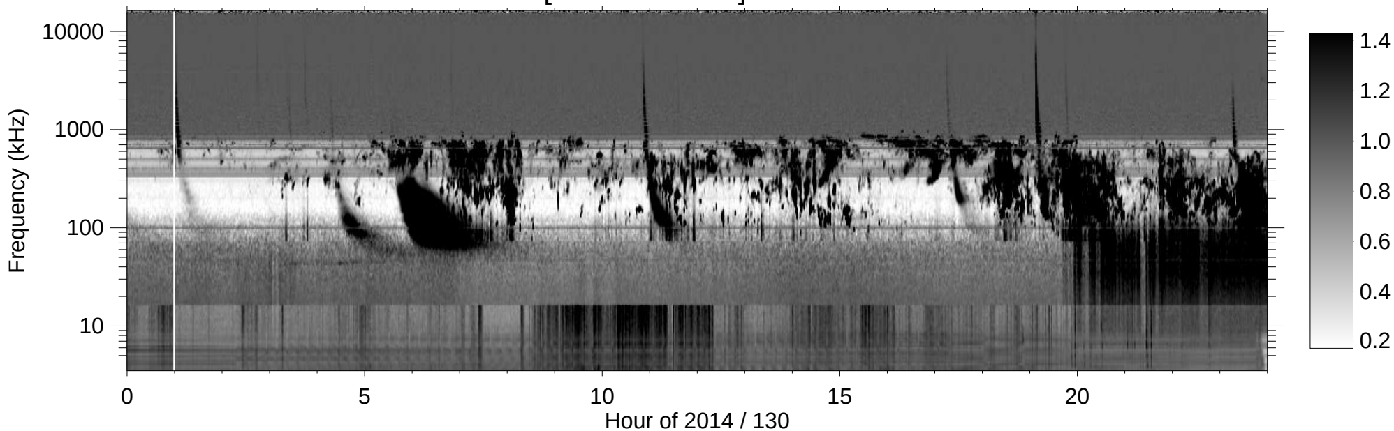
RPWS [ABCH1H2/Ex] (-B) 2014/05/10
