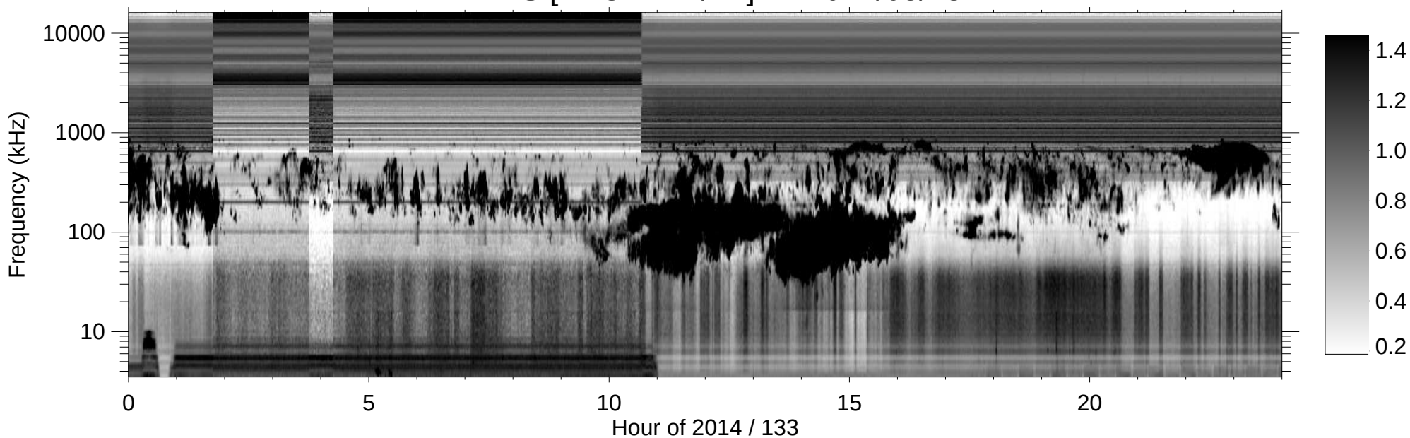
RPWS [ABCH1H2/Ex] (-B) 2014/05/13
