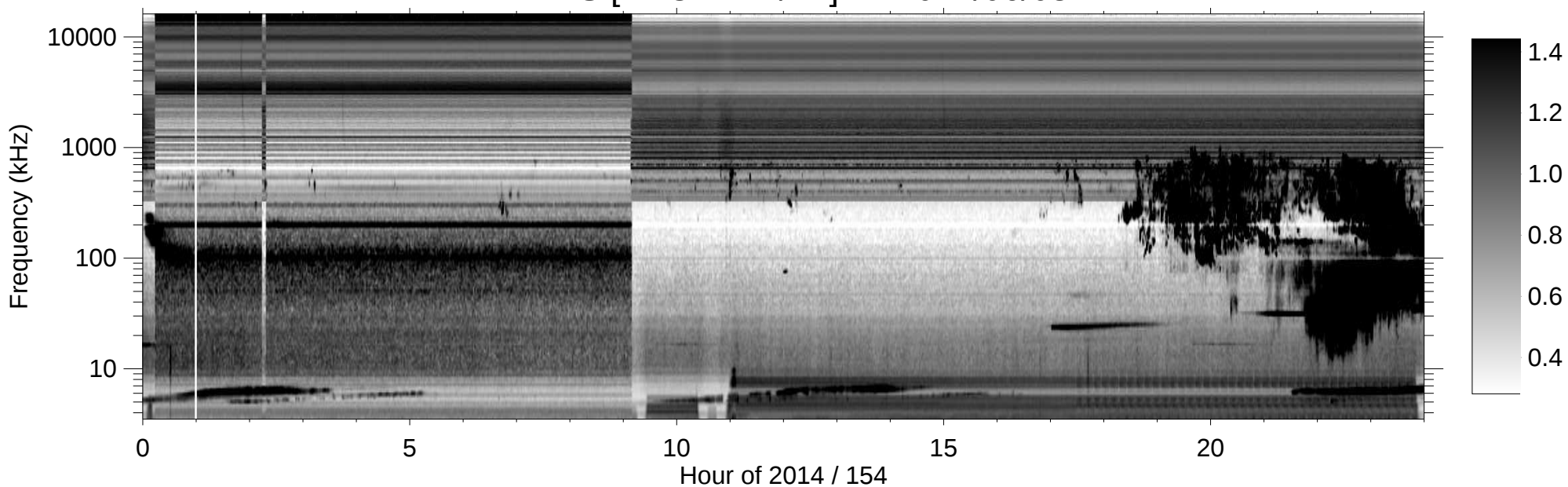
RPWS [ABCH1H2/Ex] (-B) 2014/06/03
