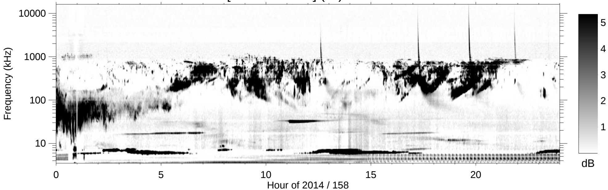
RPWS [ABCH1H2/Ex] (-B) 2014/06/07
