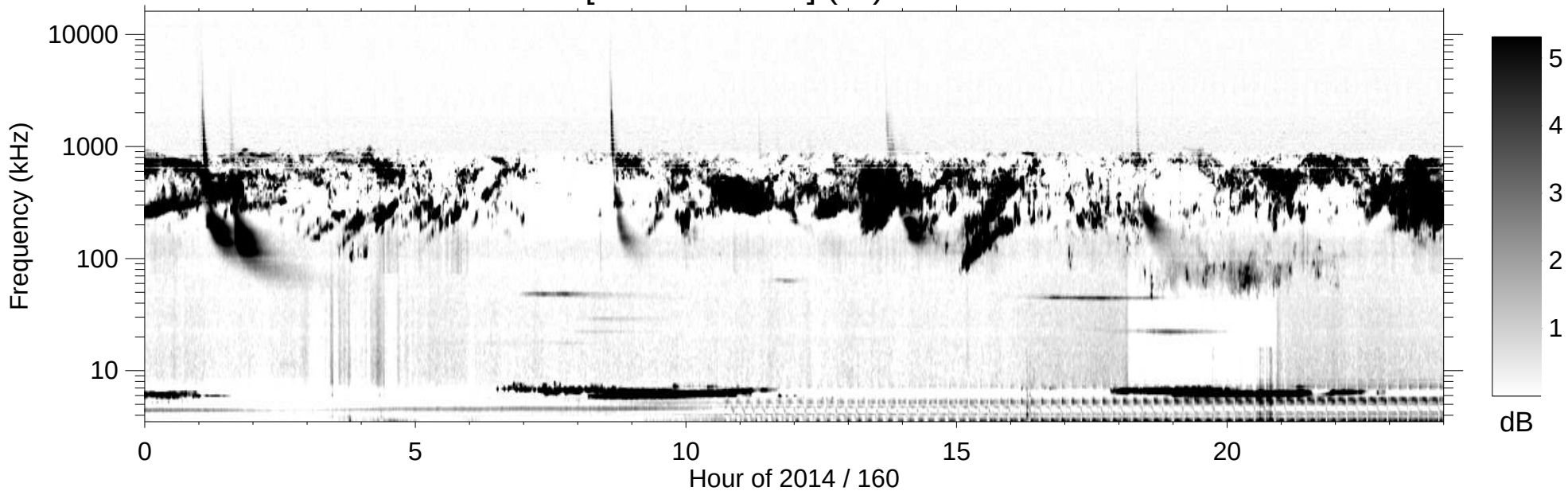
RPWS [ABCH1H2/Ex] (-B) 2014/06/09
