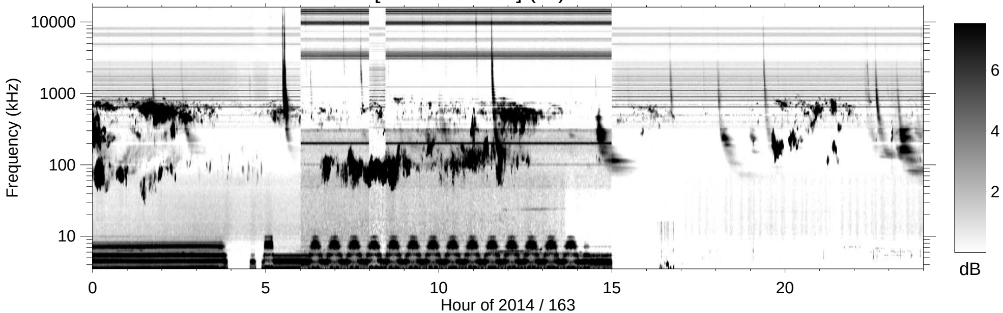
RPWS [ABCH1H2/Ex] (-B) 2014/06/12
