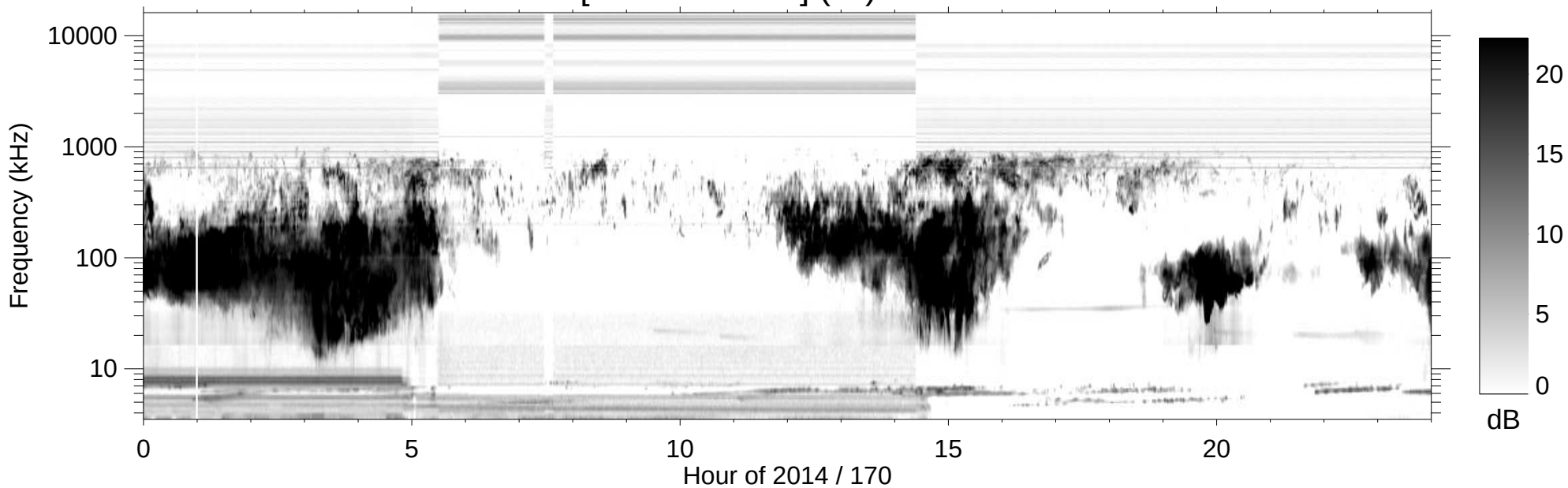
RPWS [ABCH1H2/Ex] (-B) 2014/06/19
