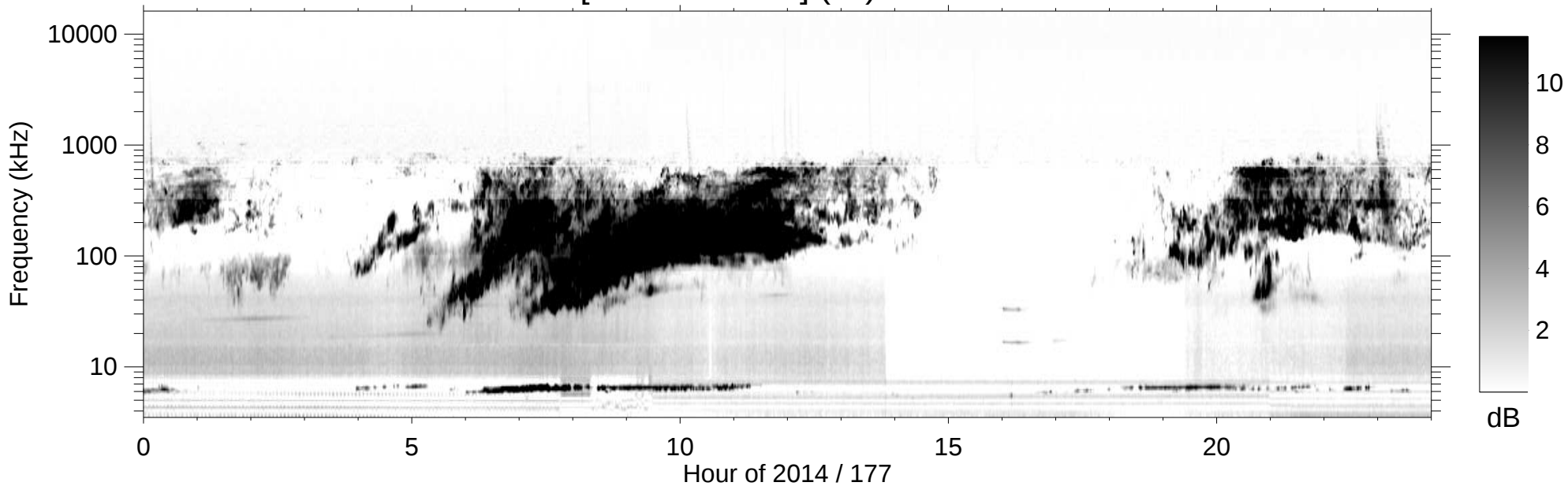
RPWS [ABCH1H2/Ex] (-B) 2014/06/26
