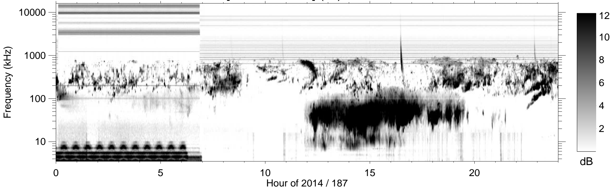
RPWS [ABCH1H2/Ex] (-B) 2014/07/06
