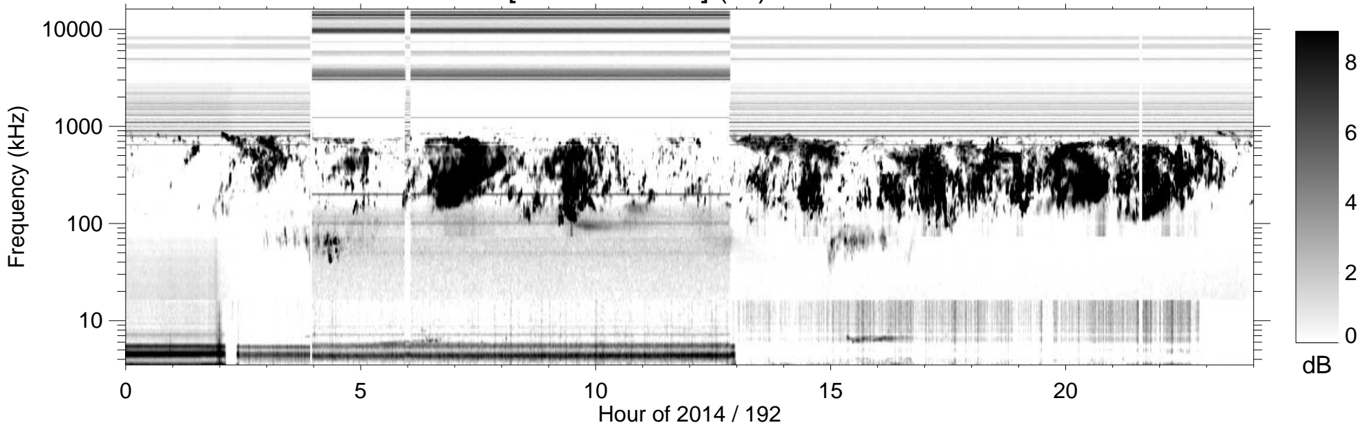
RPWS [ABCH1H2/Ex] (-B) 2014/07/11
