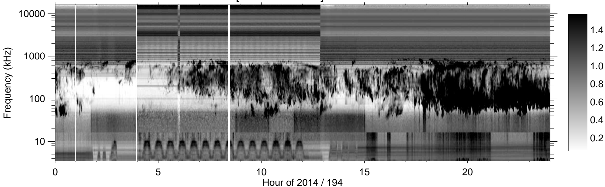
RPWS [ABCH1H2/Ex] (-B) 2014/07/13
