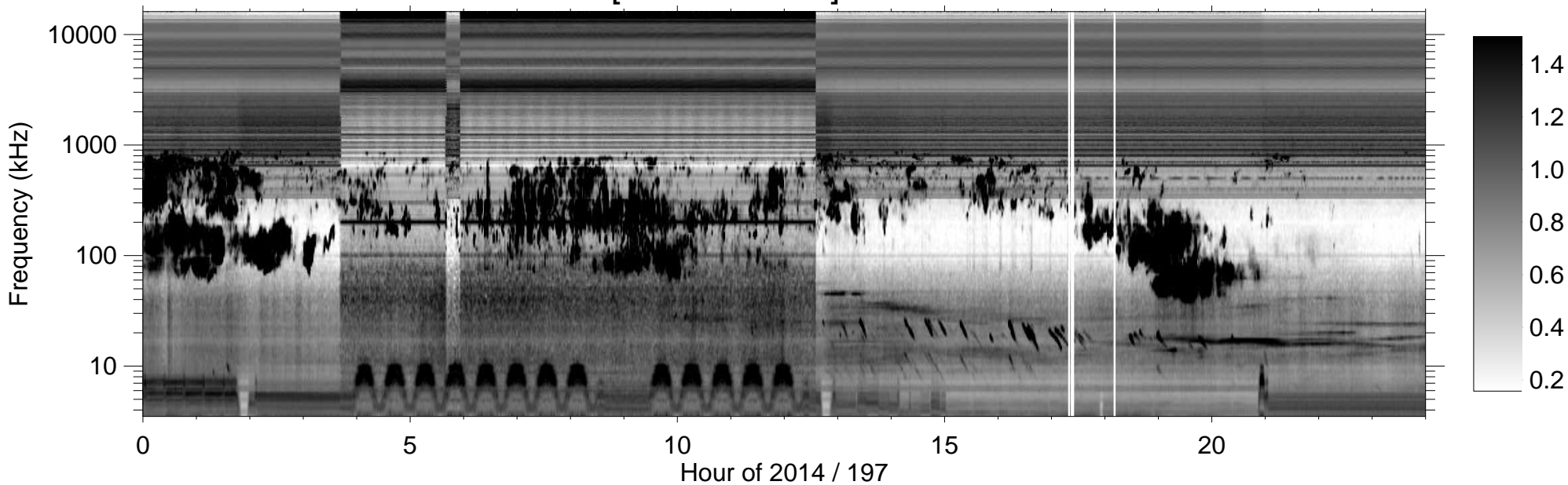
RPWS [ABCH1H2/Ex] (-B) 2014/07/16
