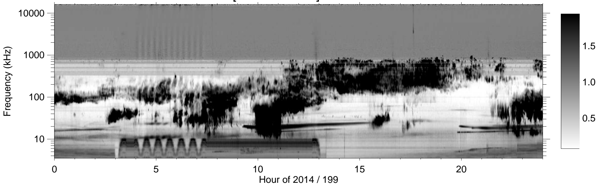
RPWS [ABCH1H2/Ex] (-B) 2014/07/18
