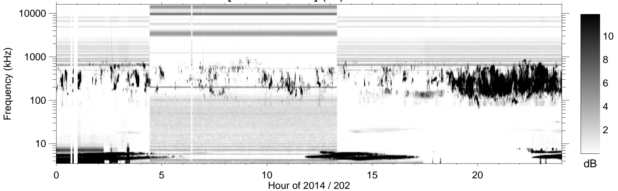
RPWS [ABCH1H2/Ex] (-B) 2014/07/21
