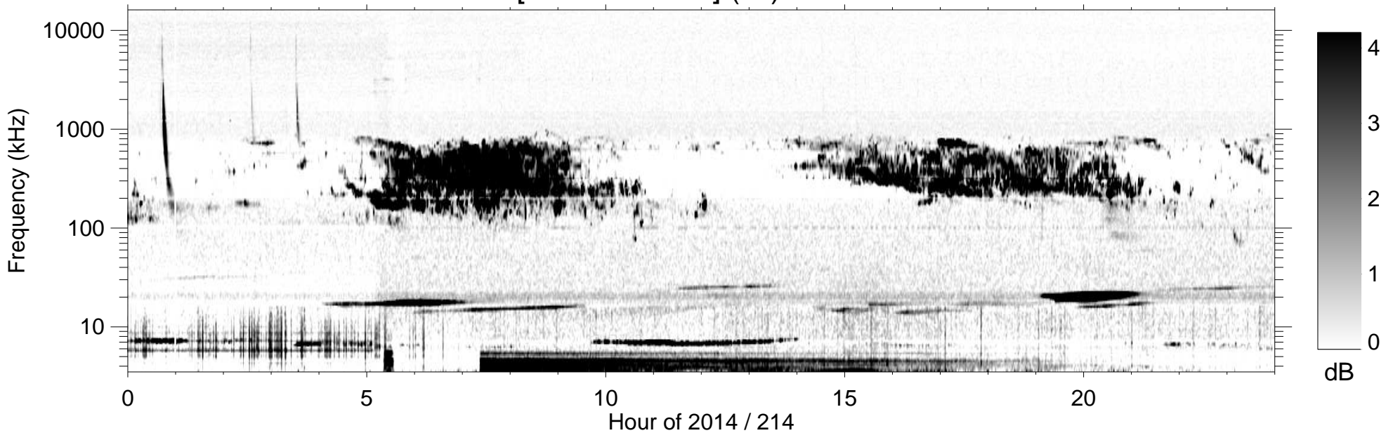
RPWS [ABCH1H2/Ex] (-B) 2014/08/02
