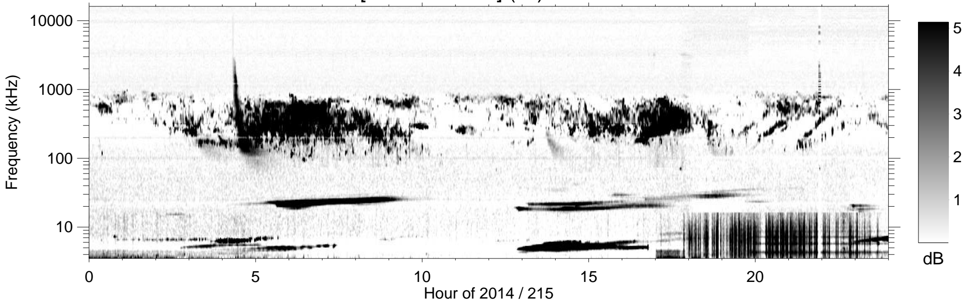
RPWS [ABCH1H2/Ex] (-B) 2014/08/03
