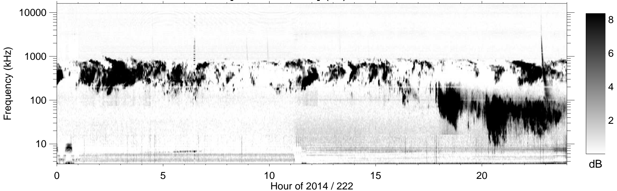
RPWS [ABCH1H2/Ex] (-B) 2014/08/10
