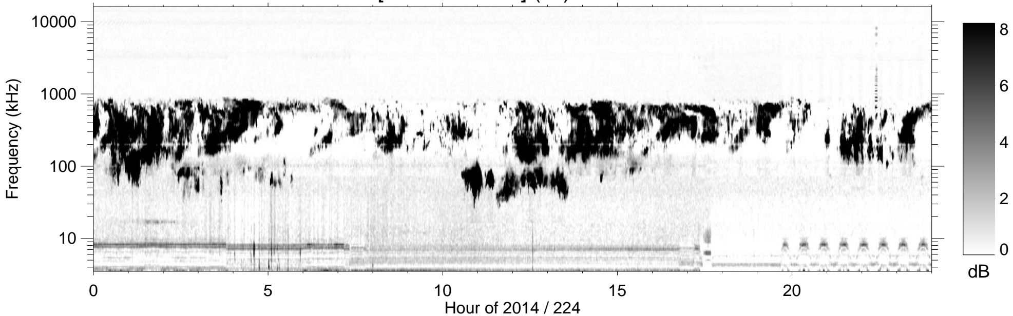
RPWS [ABCH1H2/Ex] (-B) 2014/08/12
