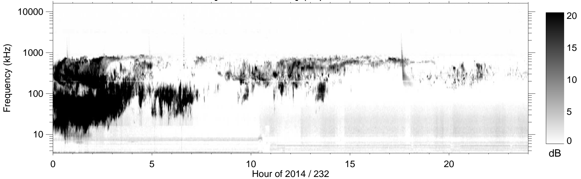
RPWS [ABCH1H2/Ex] (-B) 2014/08/20
