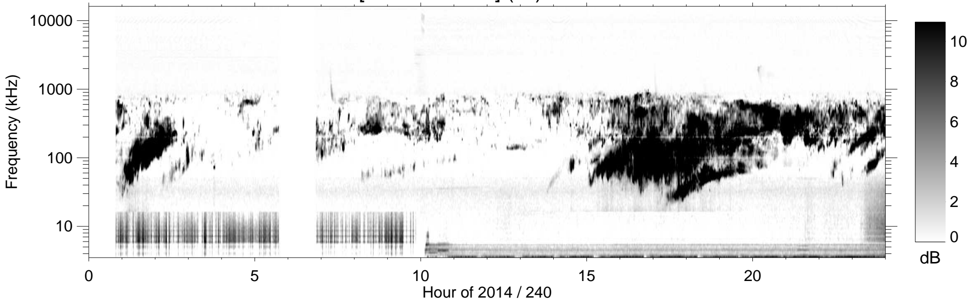
RPWS [ABCH1H2/Ex] (-B) 2014/08/28
