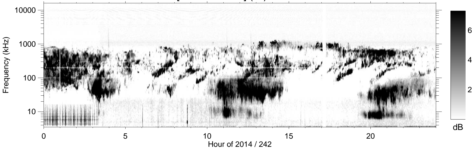
RPWS [ABCH1H2/Ex] (-B) 2014/08/30
