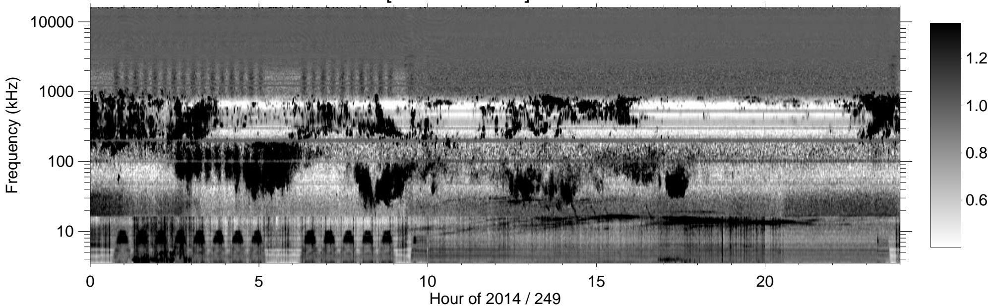
RPWS [ABCH1H2/Ex] (-B) 2014/09/06
