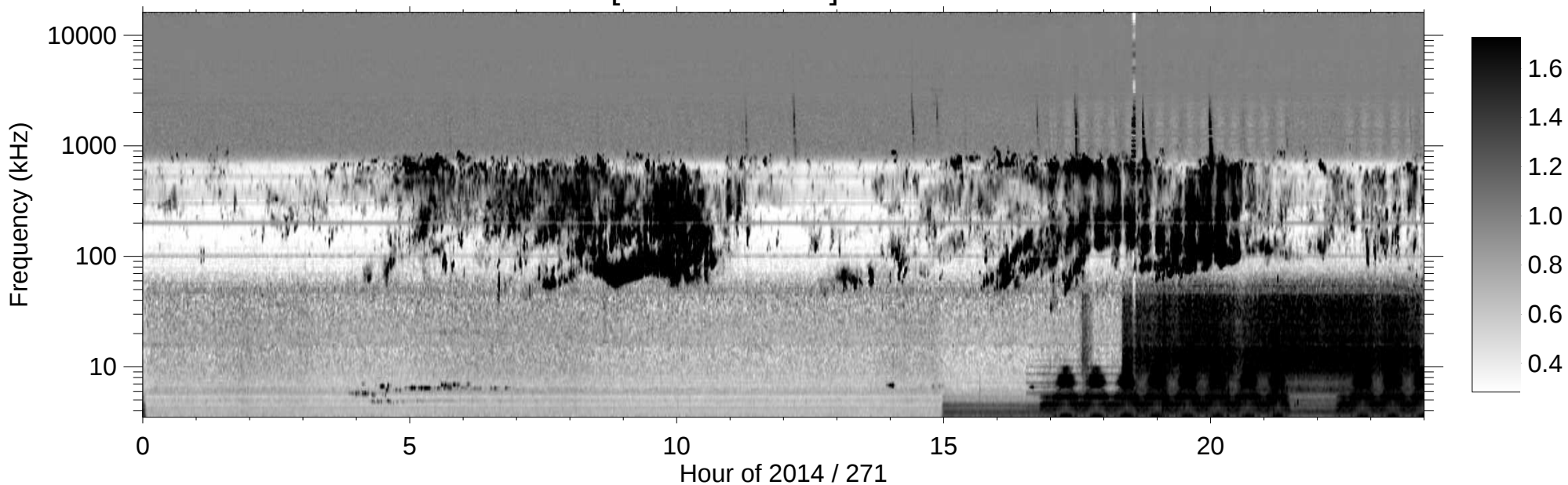
RPWS [ABCH1H2/Ex] (-B) 2014/09/28
